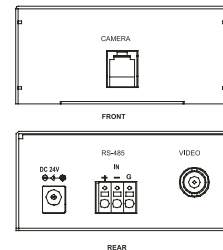
"TX1B 1-Ch Dome Interface
