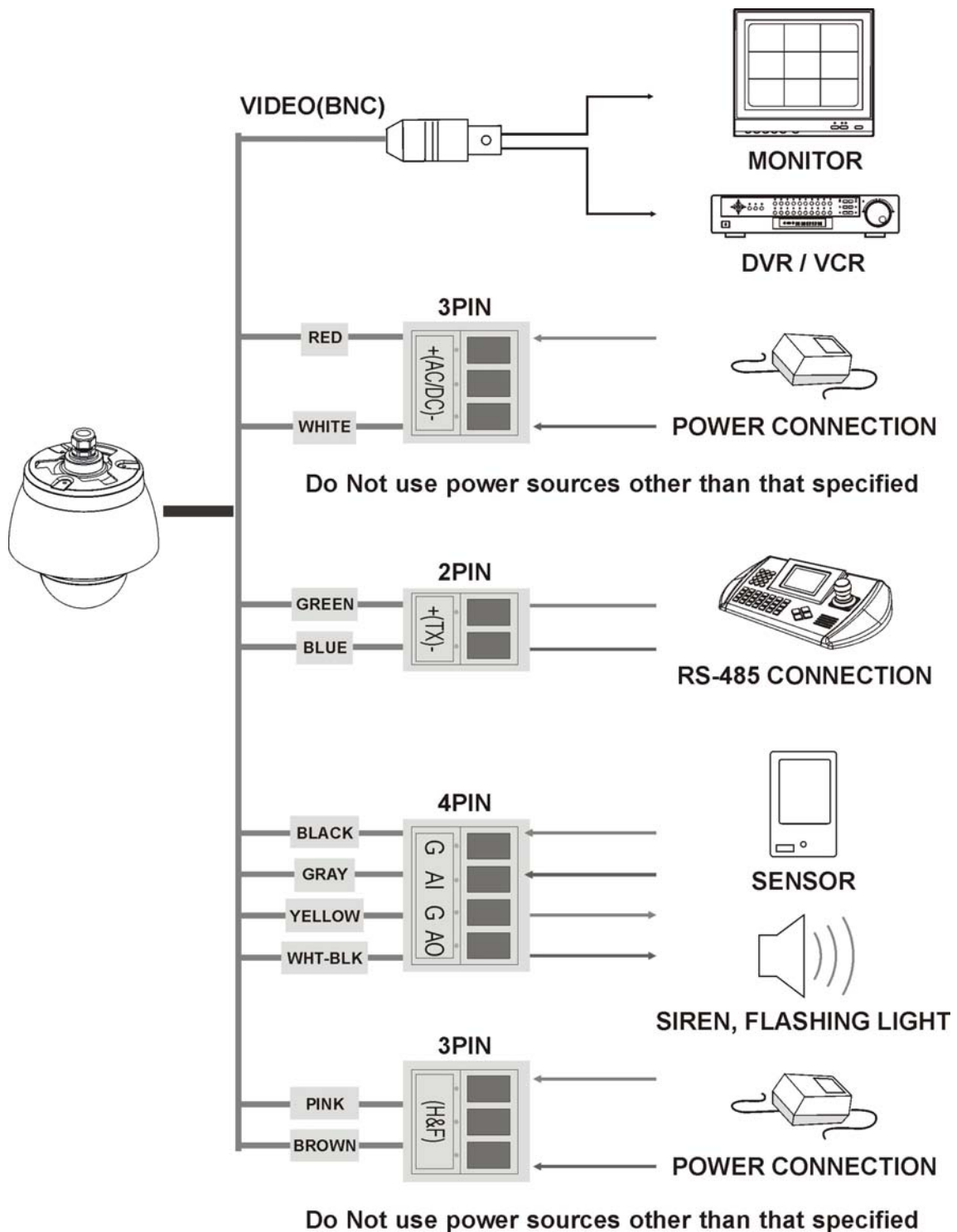
Figure 1 – Basic Installation Diagram
